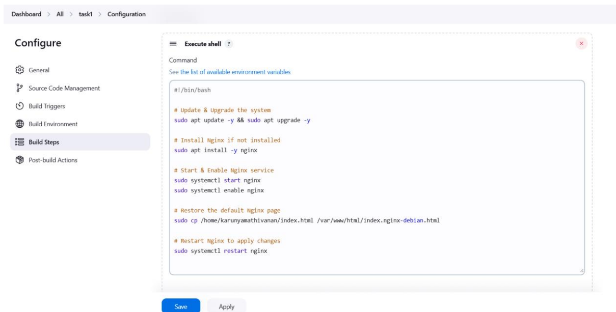
Fig 1.3 Install nginx
